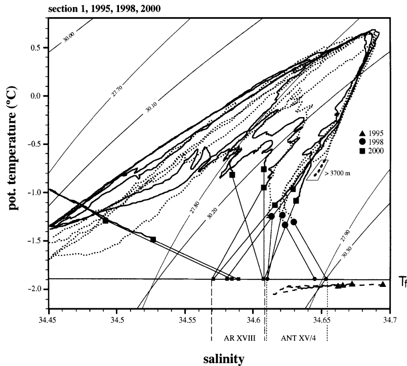
Fig. 9. Composited potential temperature vs. salinity ( \theta/S ) diagram from the continental slope off the AP for the years 1998 (dotted line/filled dots) and 2000 (solid line/filled squares), and north of the Filchner Trough for 1995 (dashed line/filled triangles). The latter covers descending Ice Shelf Water. Tangents to the end curvatures, marked by symbols for corresponding years (see insert), are drawn to identify possible source water masses at the surface freezing point ( T_f ). Vertical lines (dashed) below T_f mark the salinity ranges of the source waters for AR XVIII and ANT XV/4 with a threshold salinity of S = 34.610 . The small trapezoid represents the 1998- \theta/S space for WSBW at the base of the continental slope ( > 3700 m). Isopycnals are drawn relative to the surface and to 500 m.
