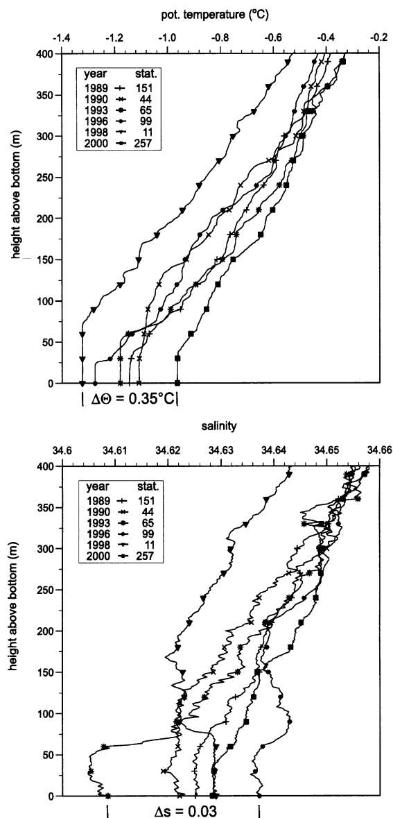
Fig. 10. Potential temperature (top) and salinity (bottom) profiles of the lowest 400 m above bottom near mooring position AWI 207 for different years listed in the insert. Maximum ranges ( \Delta ) observed so far are shown at the bottom.
